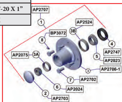
AP2707, HUB ASSEMBLY, 4 BOLT
